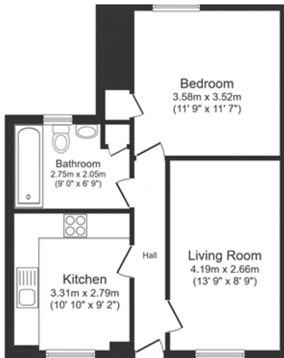
Floor Plan
